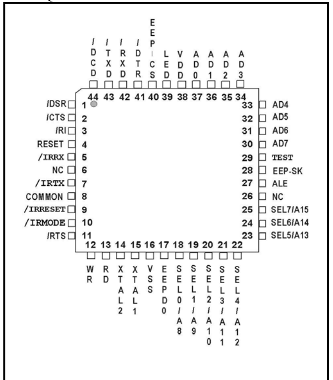
44-Pin QFP
