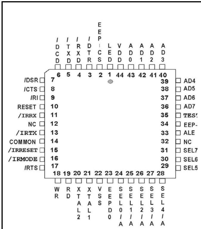
44-Pin PLCC
